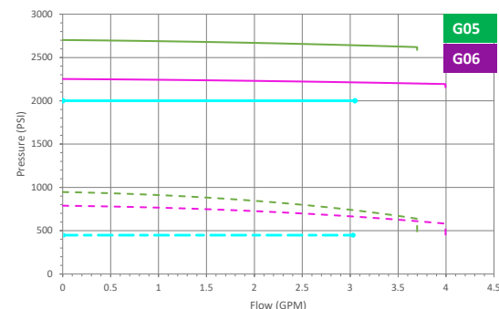
Graph B Motor A10D
