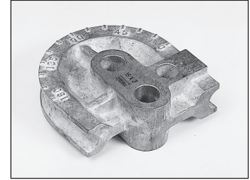
Fig. Q27 – Radius Block for use with HB632 Bender
